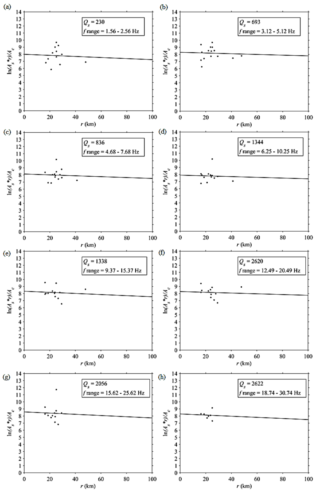
Figure 3. Decay of normalised S wave amplitudes with the r
