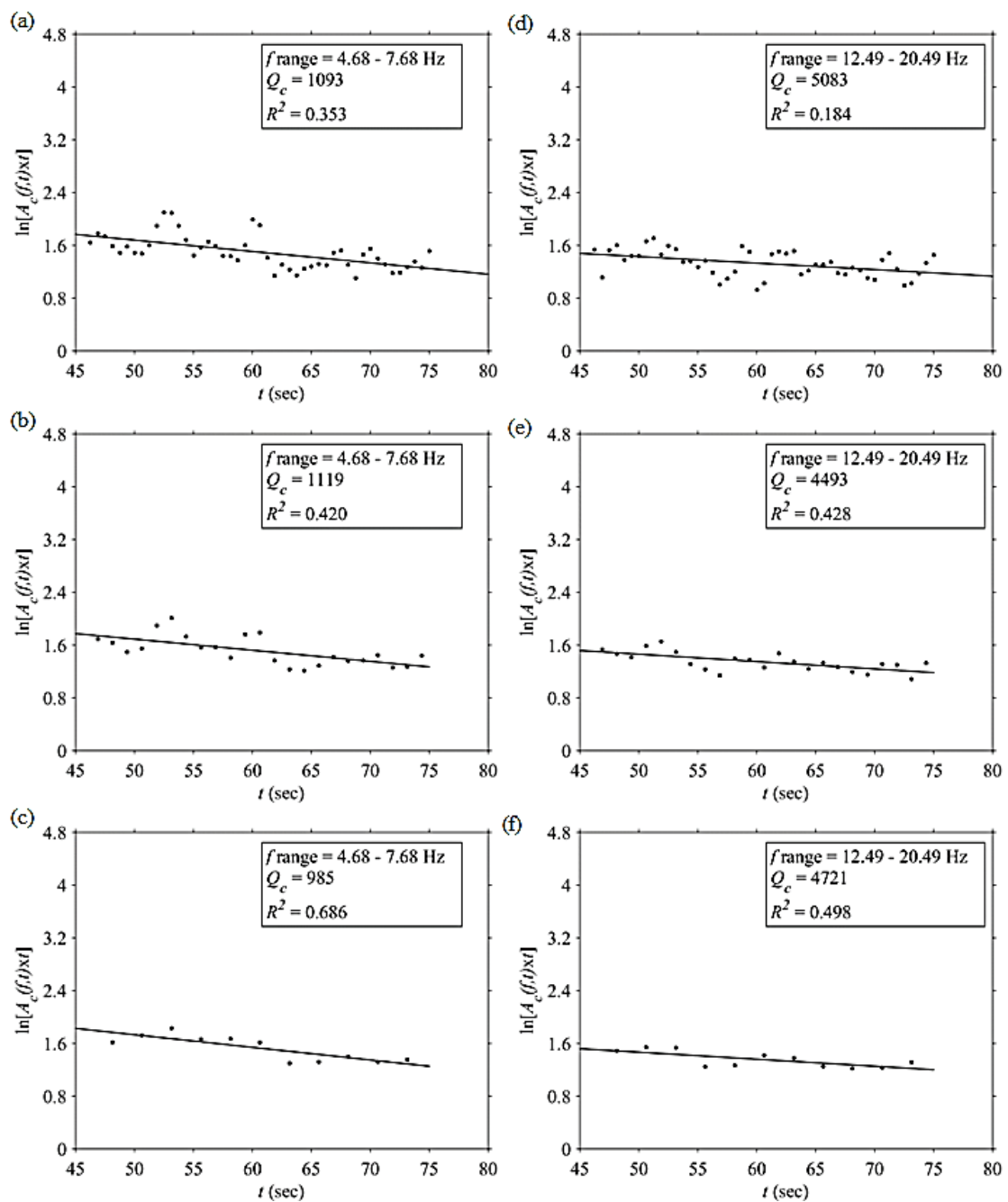
Figure 6. Coda decay envelope for two different f ranges 4.68 - 7.68 Hz and 12.49 - 20.49 Hz considering Sw values of: 1.25 s in (a) and (d); 2.5s in (b) and (e); 5s in (c) and (f)
