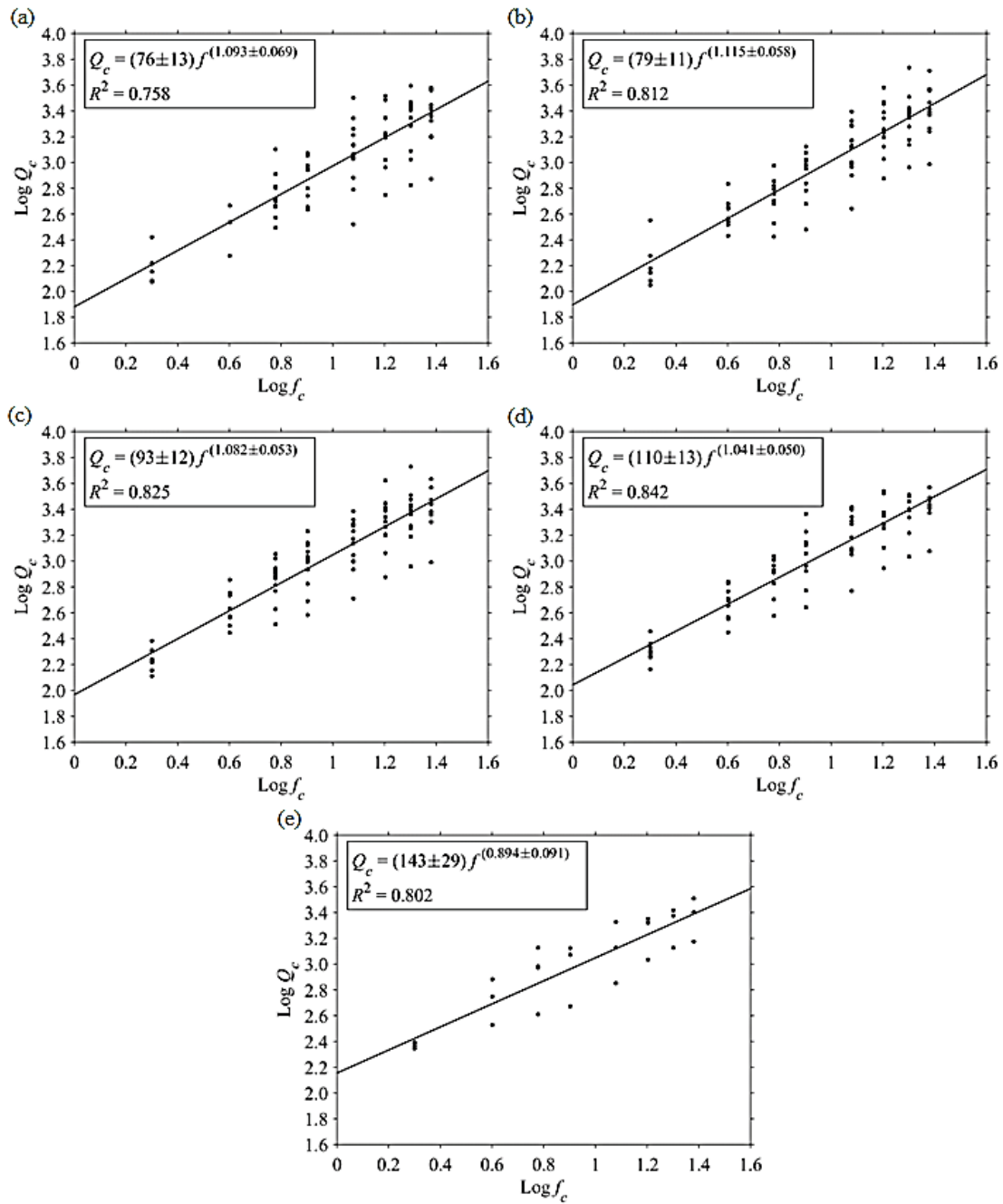
Figure 7. Q - f correlation for coda wave in Garhwal region considering cw (a) 20s, (b) 25s, (c) 30s, (d) 35s, (e) 40s
