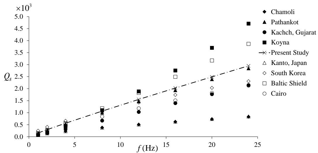
Figure 9. Comparison of S wave attenuation in the present study with the other active tectonic areas in India and worldwide
