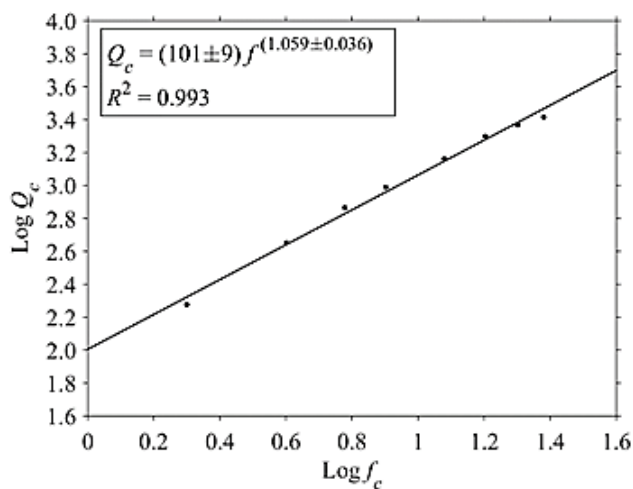
Figure 11. Average Q - f correlation for coda wave in the Garhwal region
