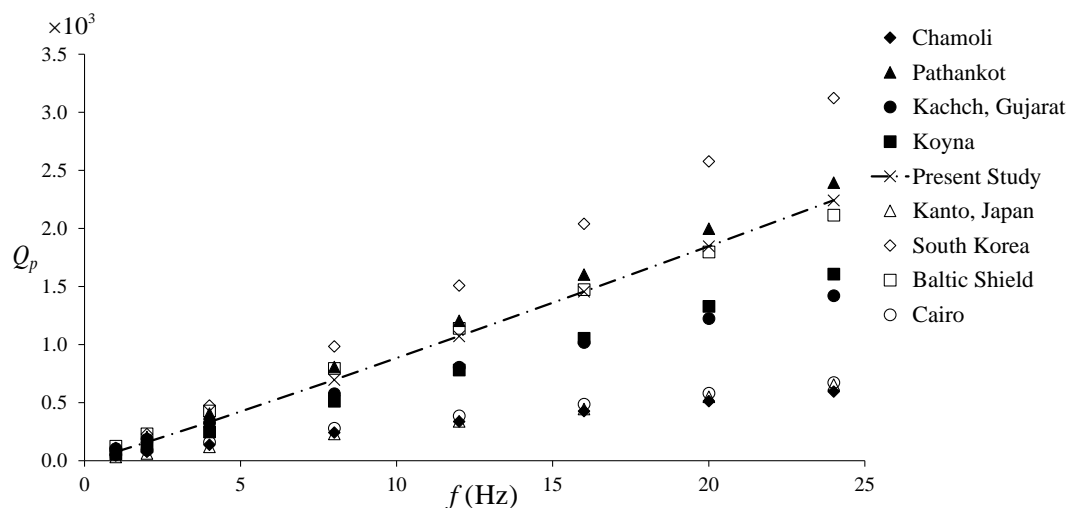
Figure 8. Comparison of P wave attenuation in the present study with the other active tectonic areas in India and worldwide
