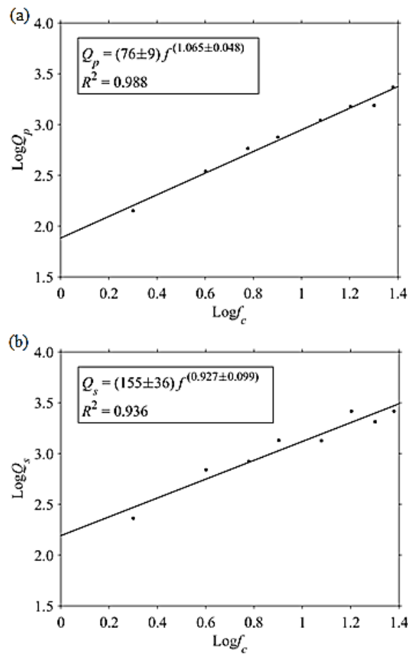
Figure 4. Q - f correlation for P and S wave in Garhwal region
