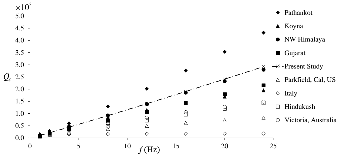
Figure 12. Comparison of coda wave attenuation in the present study with the other active tectonic areas in India and worldwide
