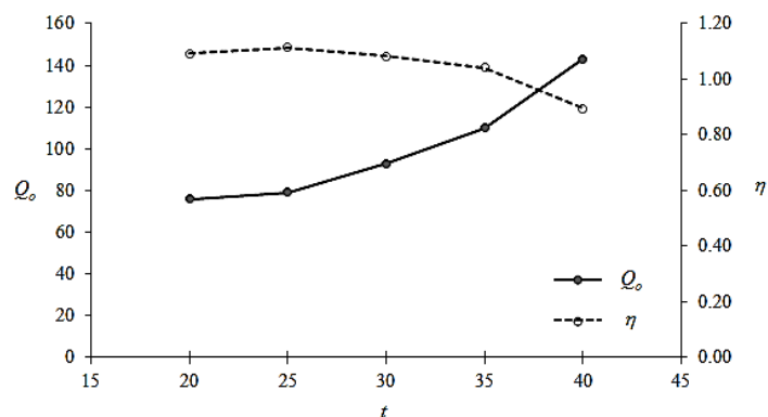
Figure 10. Variation in Q_o and \eta values with the increasing t
