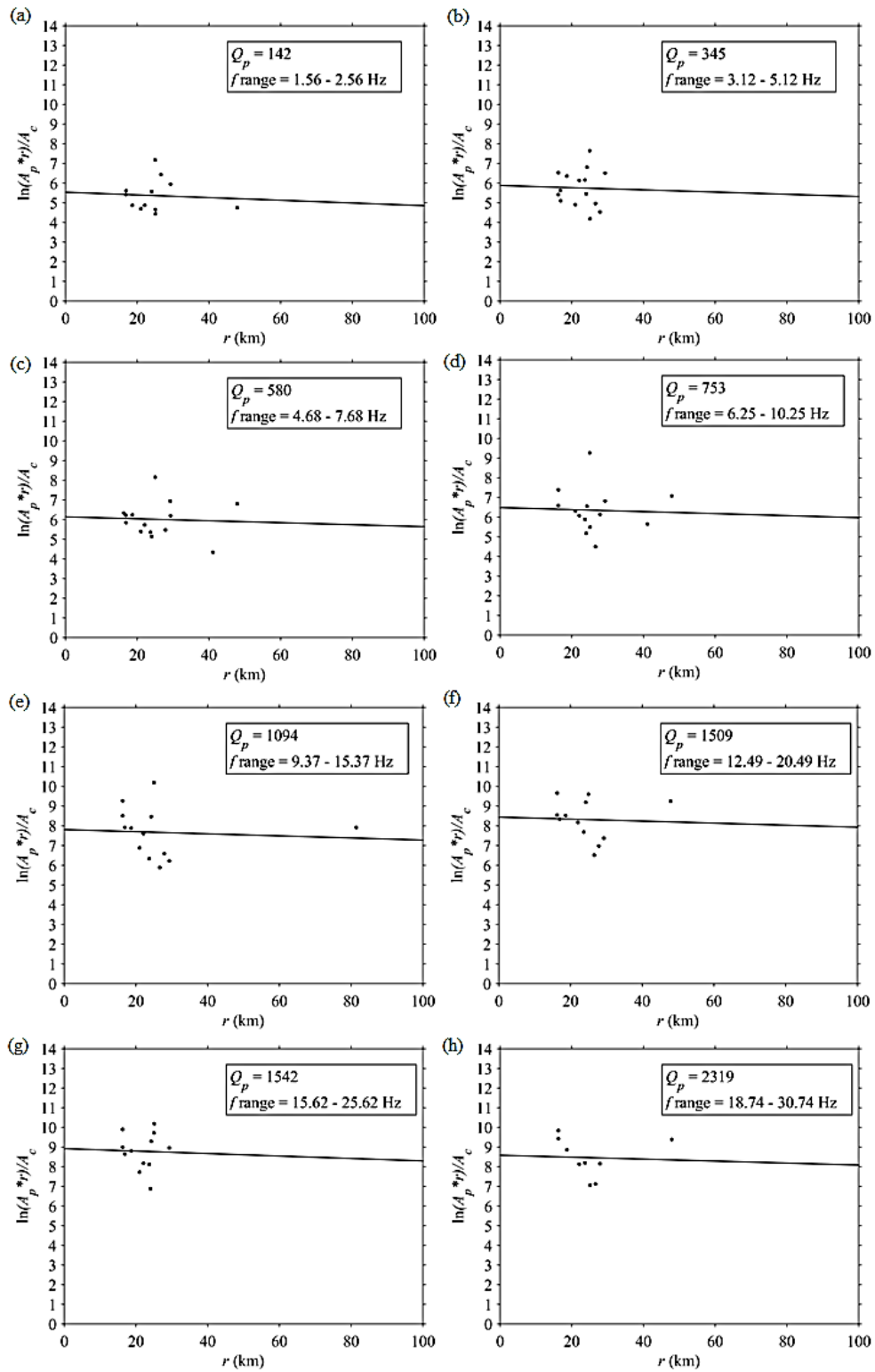
Figure 2. Decay of normalised P wave amplitudes with the r
