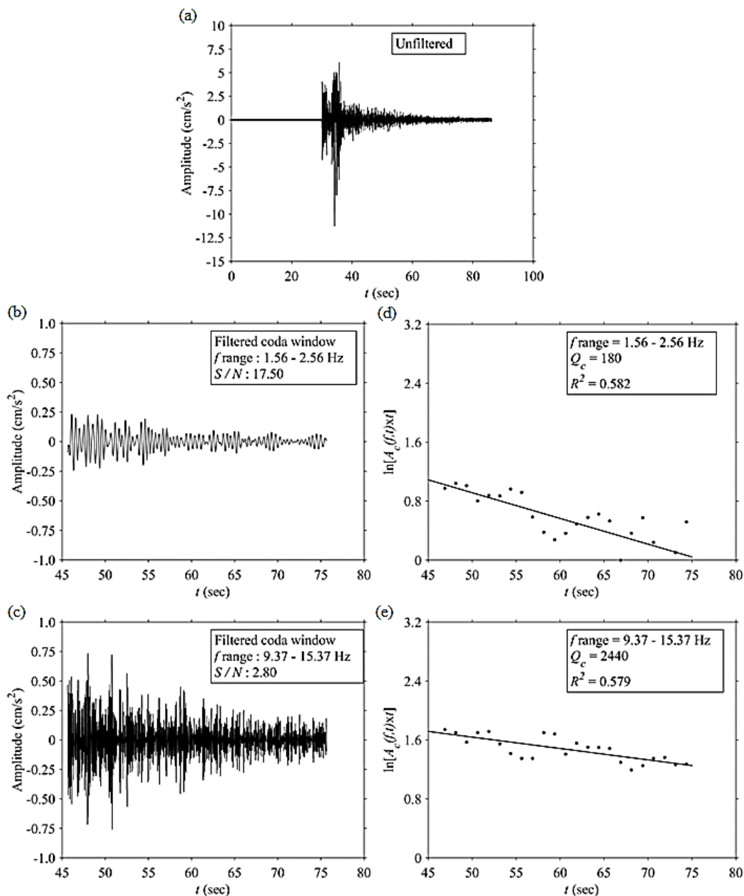
Figure 5. (a) Unfiltered seismogram of 4.6 M_w EQ on 01-05-2010 recorded at Bageshwer station, Garhwal (29.831 N & 79.77 E), (b) and (c) shows the filtered coda window at 1.56 – 2.56 Hz and 9.37 – 15.37 Hz, (d) and (e) shows the corresponding coda decay envelope and Q_c values at 1.56 – 2.56 Hz and 9.37 – 15.37 Hz
